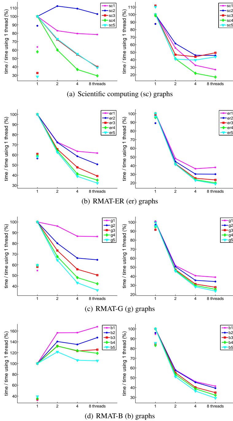
Fig. 1. Scalability results on the two parallel SL ordering algorithms. Left column: Algorithm 2 (SL-Regular). Right column: Algorithm 3 (SL-Relaxed). The plots show runtimes normalized by the runtime when 1 thread is used; the raw numbers for the case of 1 thread are listed in Table 3. Also shown are data points corresponding to runtime of the pure sequential algorithm normalized by the runtime of the parallel algorithm run on 1 thread.
